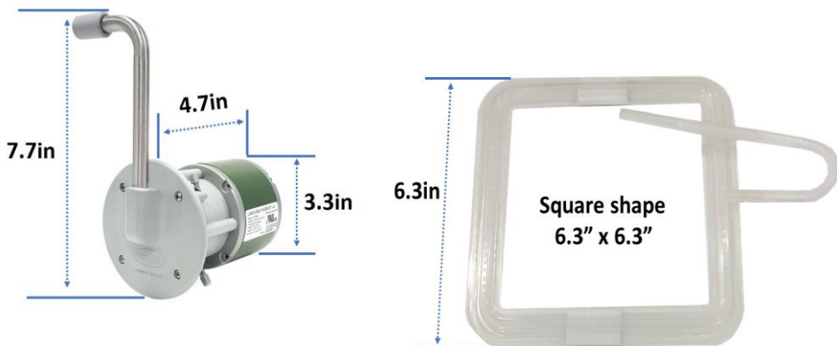
Figure 2. Motor dimensions
