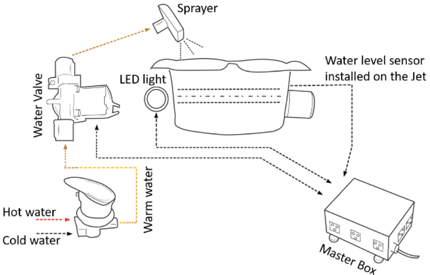
Fig.1: Connection Diagram
