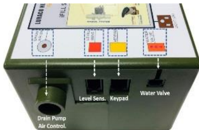
Fig. 3: Input and Output Control Ports
