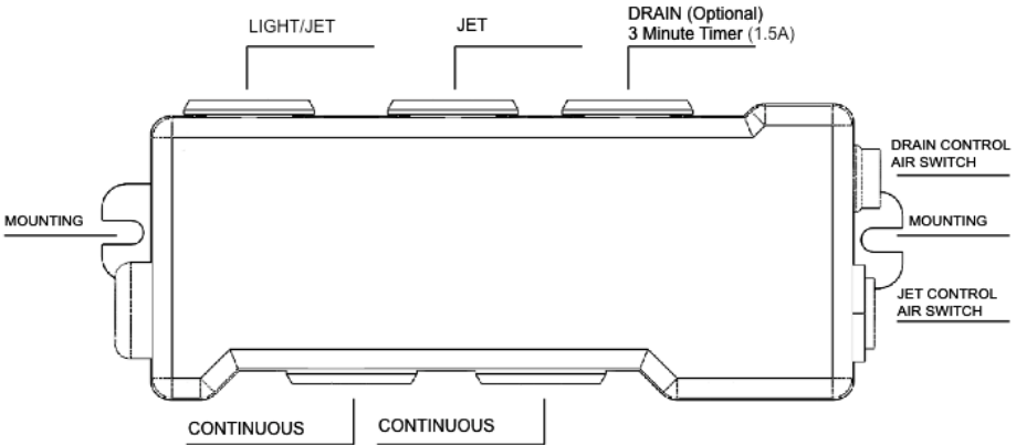
Fig.1 Port Designation
