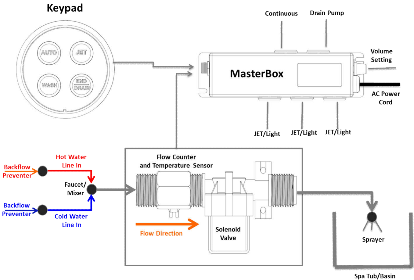
Fig.1: Connection Diagram
