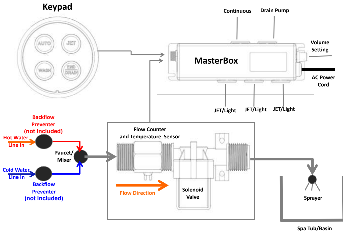
Fig.1: Connection Diagram
