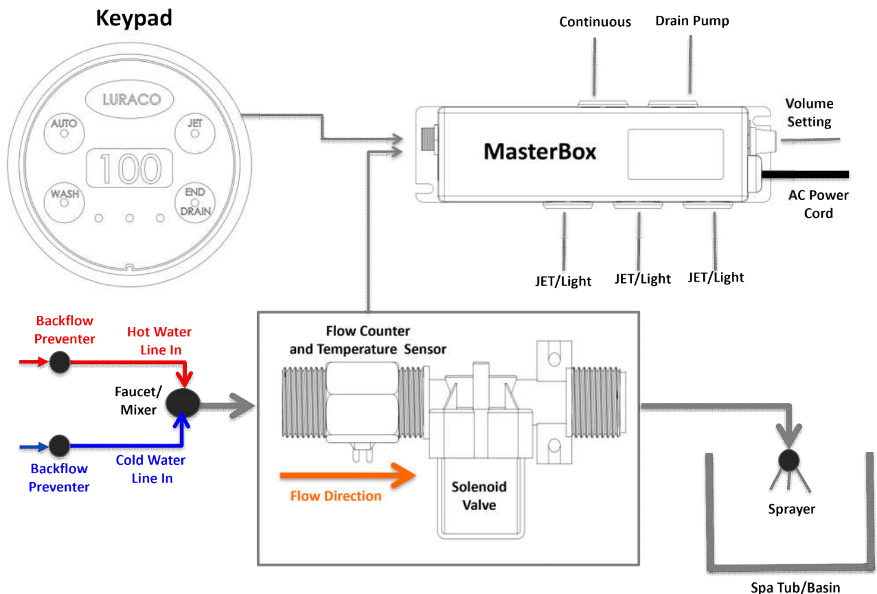
Fig.1: Connection Diagram
