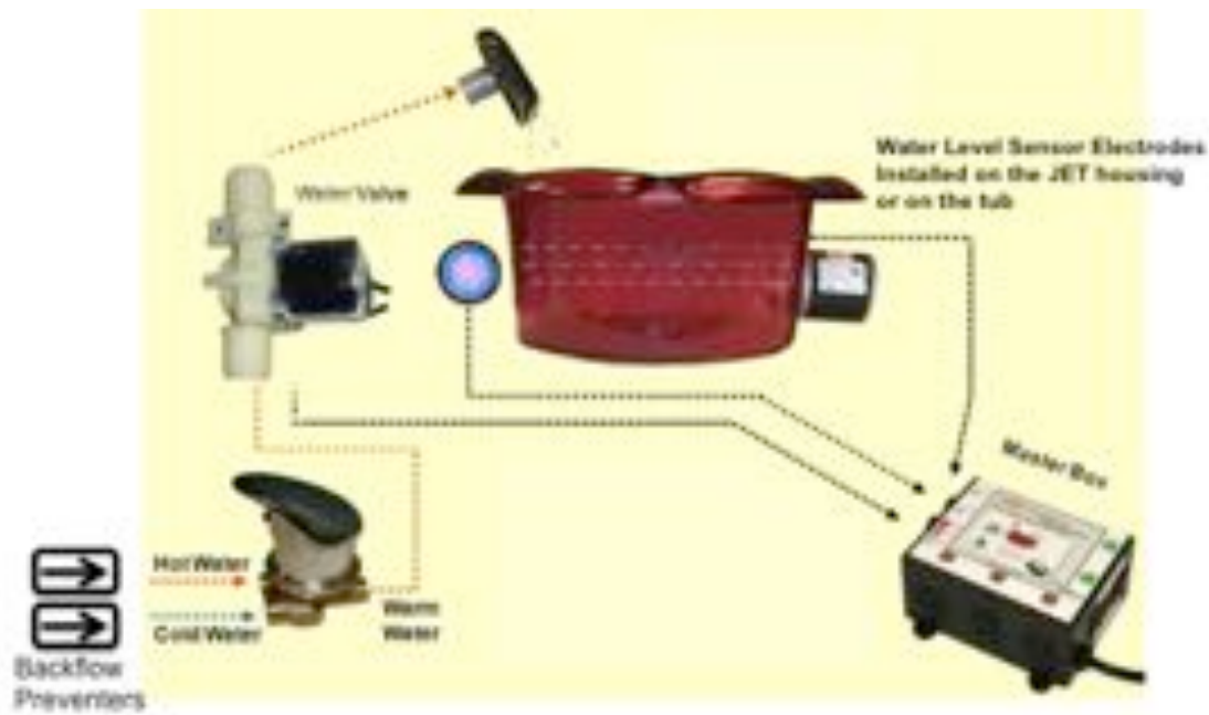
Fig.1: Connection Diagram
